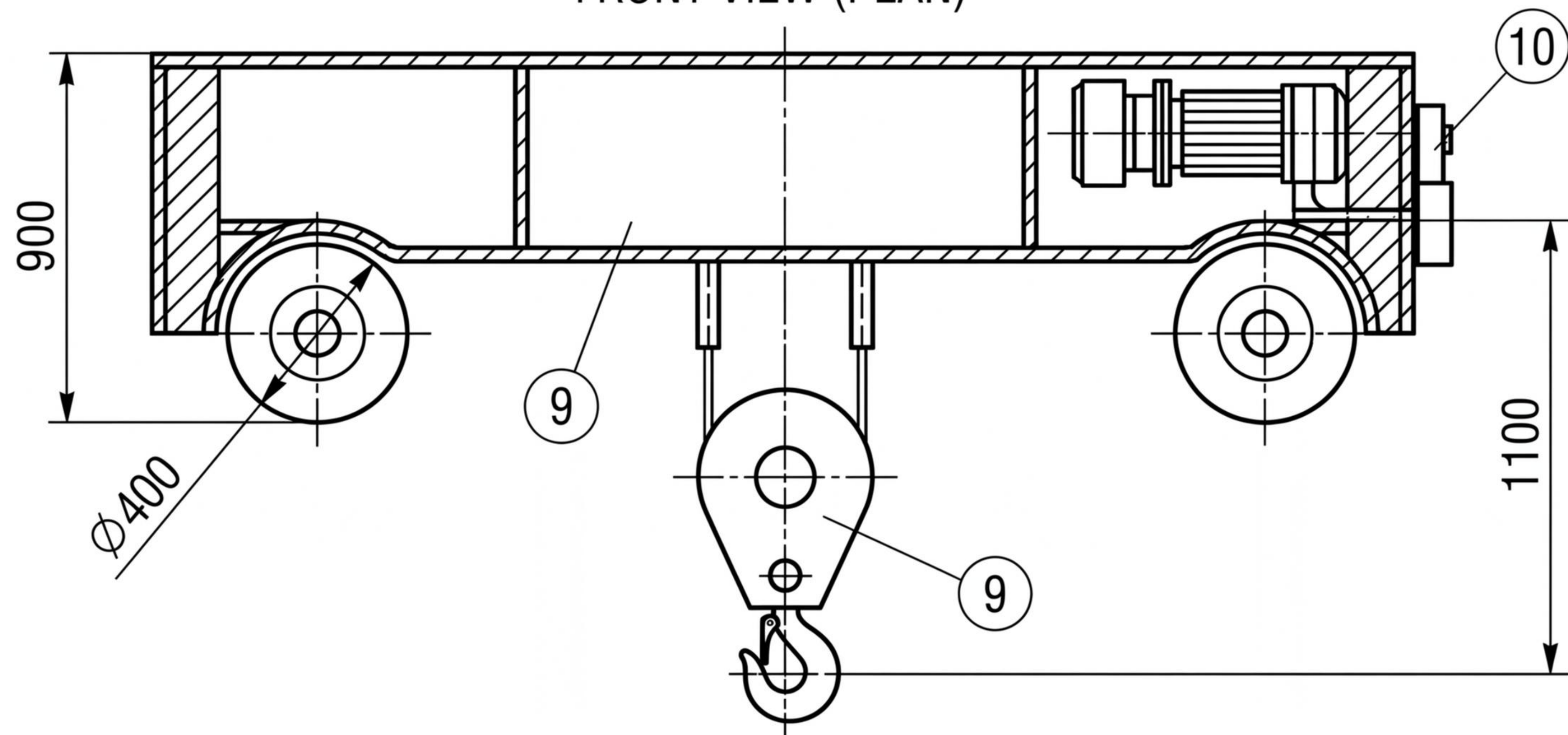
FRONT VIEW (PLAN)
