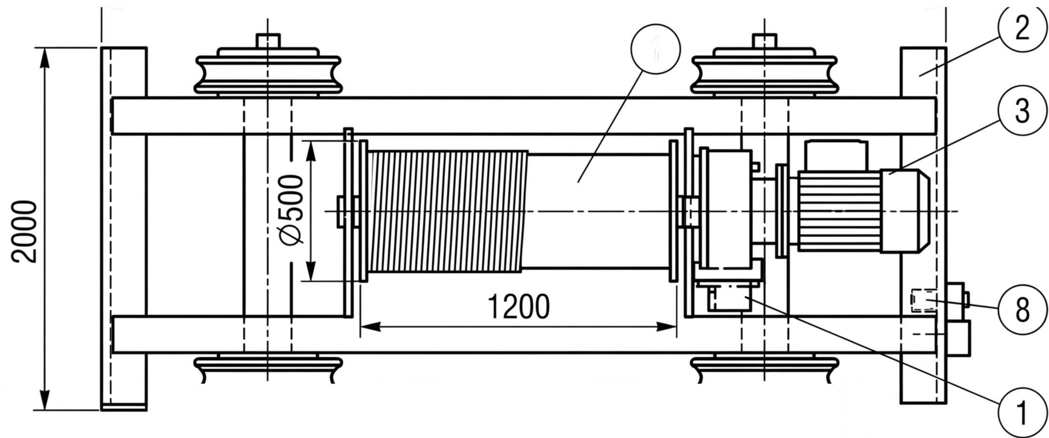
FRONT VIEW (PLAN)
